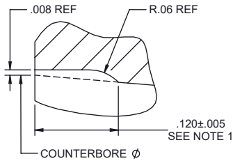
BENCHMARK DETAIL
